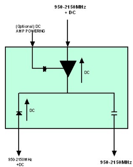
Typical Configuration
